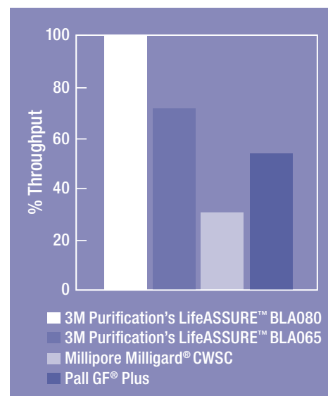
Figure 11 – Throughput Comparison
