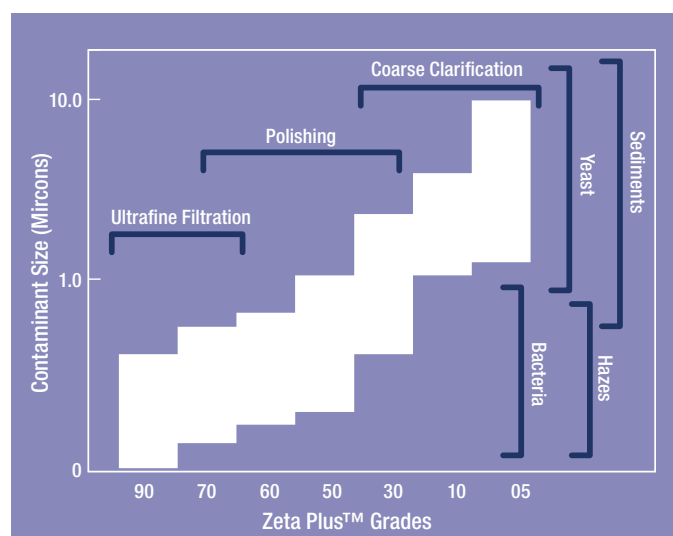
Figure 6 – Filter Grades
